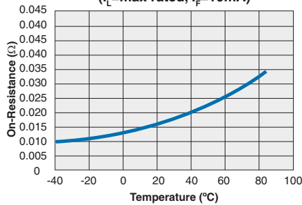
CPC1709 Typical On-Resistance vs. Temperature ( I_L = \text{max rated} , I_F = 10mA )
