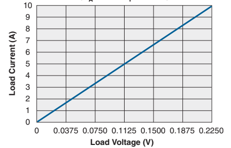
CPC1709 Typical Load Current vs. Load Voltage ( T_A = 25^\circ C , I_F = 10mA )
